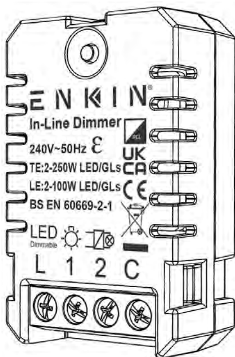
IDM250 Enkin 250W Universal In-Line LED dimmer
